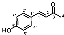
E -1-(4'-hydroxyphenyl)but-1-en-3-one 1
